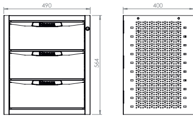
Base with 3 drawers Dimensions: 490x400x564mm
